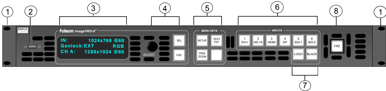
Figure 2-1. ImagePRO-II Front Panel
