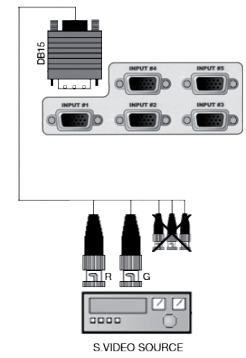
DB15 or 2xBNC
