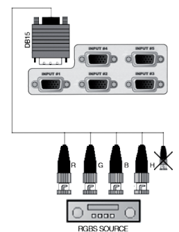
DB15 or 4xBNC
