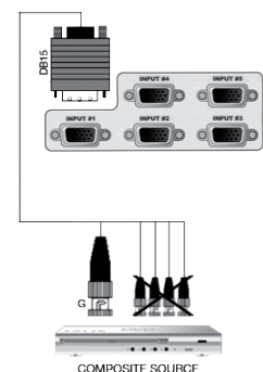
DB15 or 1xBNC
